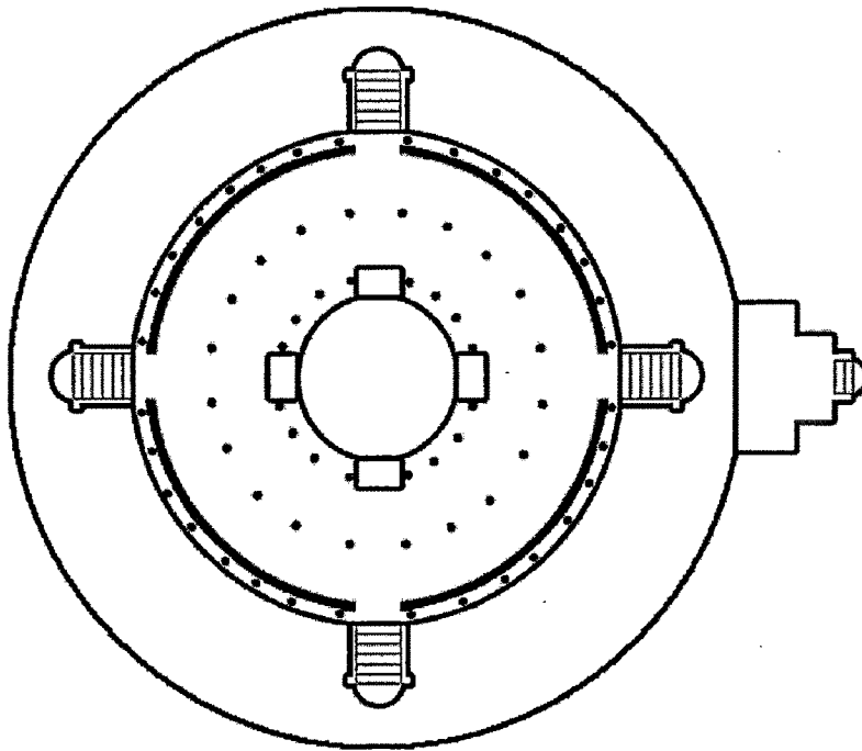
36. GROUND PLAN VATADAGE, SRI LANKA
