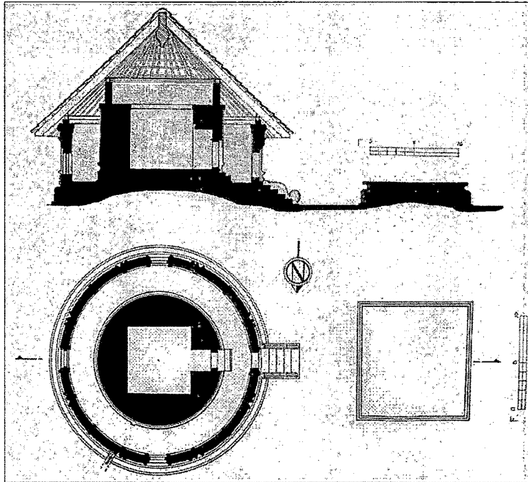
21. SECTIONAL ELEVATION OF A KERALA TEMPLE [NARAYAN KANNUR TEMPLE, RAMANTALI, KANNUR DISTRICT]
