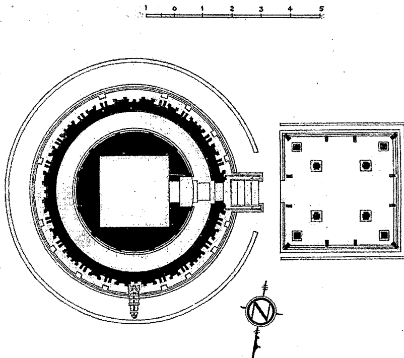
43. PLAN, VRTTAKARA SRI KOIL , [VADAKKUNNATHA TEMPLE, TRISSUR DISTRICT]
