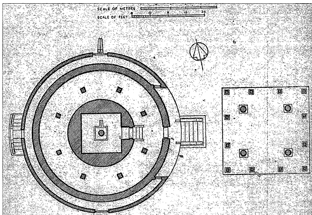
69.PLAN, KAVIYUR [ACCORDING TO H SARKAR]
