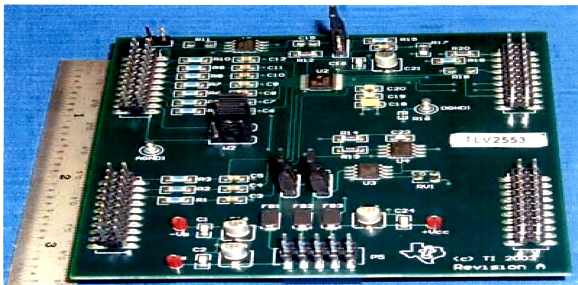
Photo A-I.3: TLV 2553 EVM (11 – input Analog to Digital Converter)
