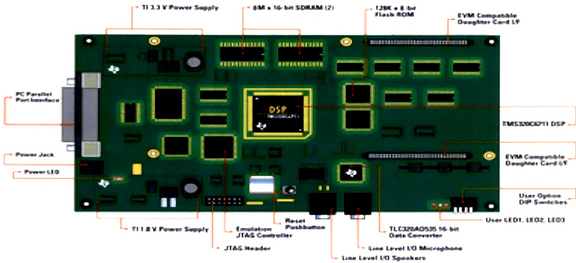
Photo A-I.1: TMS 320C6711 DSP Starter Kit
