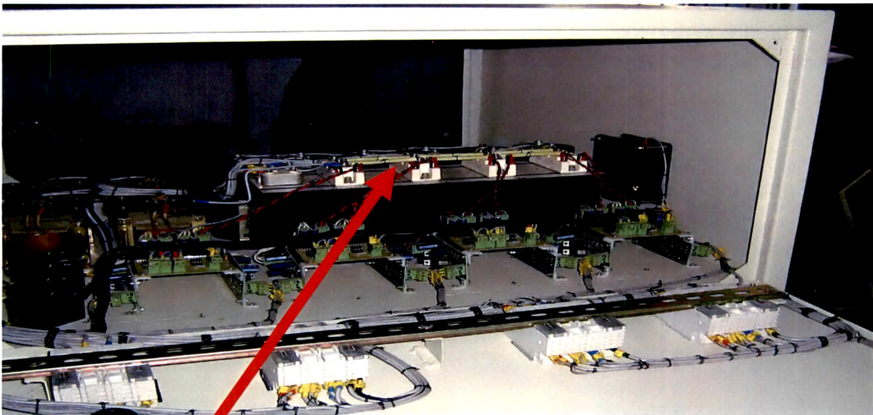
Photo A-II.6 Power module for 3- \phi Four wire configuration
