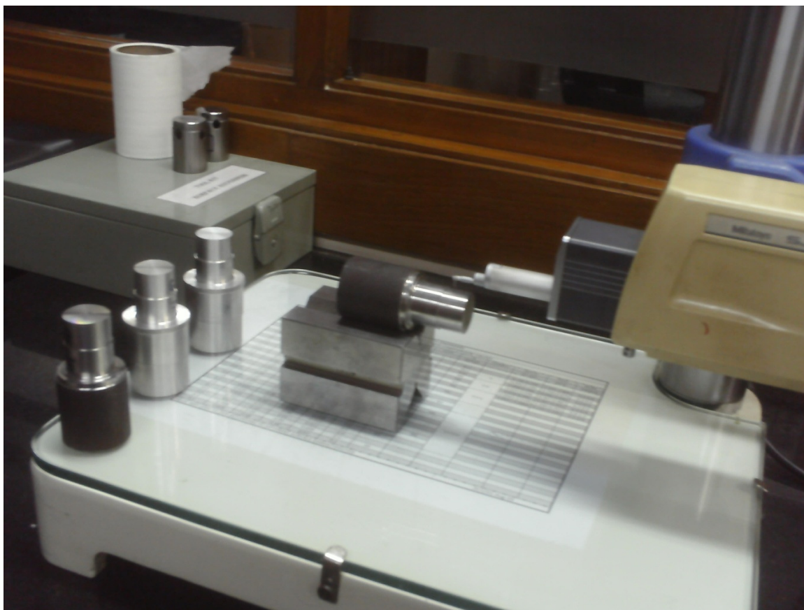
Fig. 2 Surface Roughness measurement on SJ-400 (Mitutoyo make) at G.M.Export Pvt.Ltd, Rajkot
