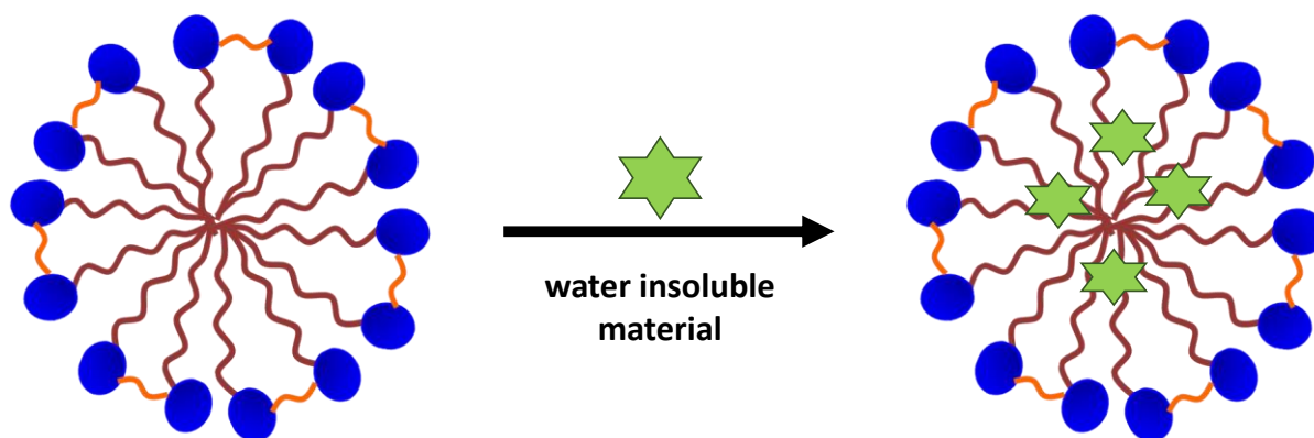
Scheme 2. Schematic representation of solubilization of hydrophobic material in micellar aggregate
