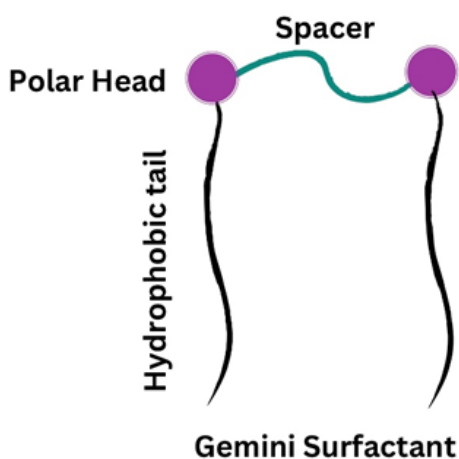
Scheme 1. Schematic representation of gemini surfactant.
