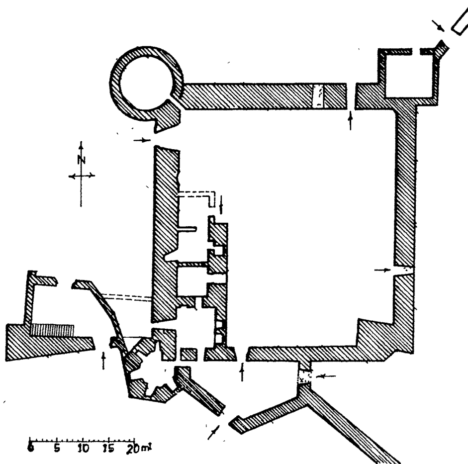
FIG. 2 G.F. PLAN OF FORTRESS
