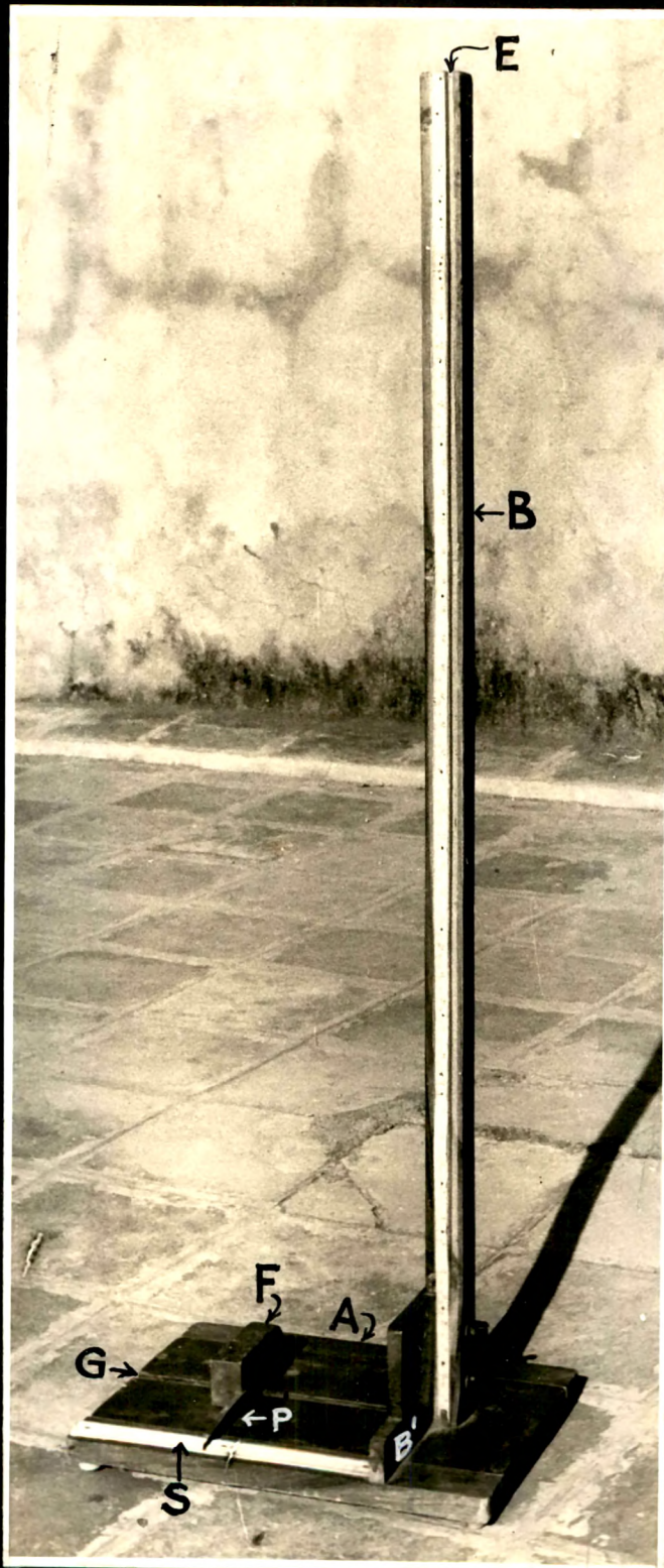
PLATE 1. Measuring Platform and rod with scale.
