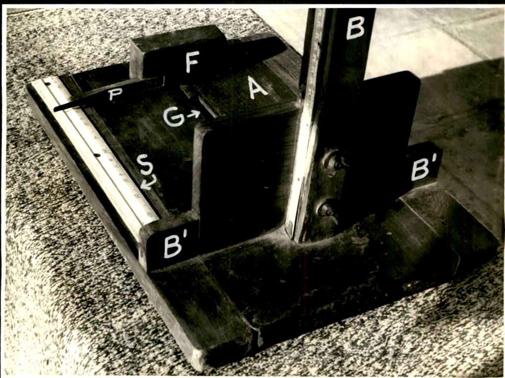
PLATE 2. Close-ups of the Measuring Platform and rod to show details. (see pp. 82, 83 and 84 of Chapter III).
